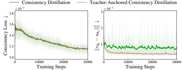
Figure 3: Training curves of two distillation methods: consistency loss (Left) and squared distance between the student’s velocity v_{\theta_S} and the teacher’s average velocity towards the clean endpoint u_{\theta_T} (Right).
