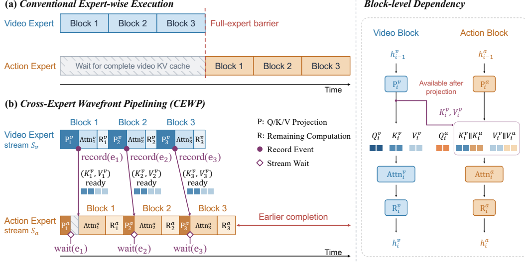
Figure 4: Comparison of expert execution schedules. (a) Conventional execution waits for the complete video KV cache. (b) Cross-Expert Wavefront Pipelining releases block-wise KV cache entries after projection and synchronizes only before action attention consumes them, overlapping the Video and Action Experts.
