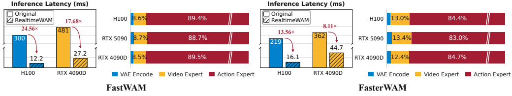
Figure 1: Inference efficiency of Fast-WAM (left) and Faster-WAM (right) across diverse hardware. Vertical bars compare inference latency between the original models and RealtimeWAM, while stacked bars show the runtime proportions of key components.
