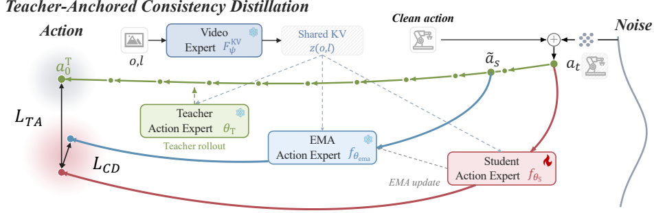
Figure 2: Overview of Teacher-Anchored Consistency Distillation (TACD). The frozen Video Expert provides shared KV conditioning, while the action student is trained with local consistency supervision and a teacher-anchored constraint derived from the frozen teacher’s multi-step rollout.
