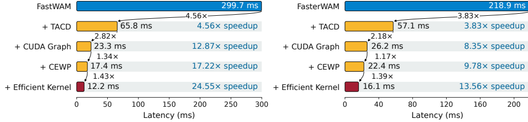
Figure 5: Inference latency of RealtimeWAM built on Fast-WAM (left) and Faster-WAM (right) on a single NVIDIA H100 GPU.
